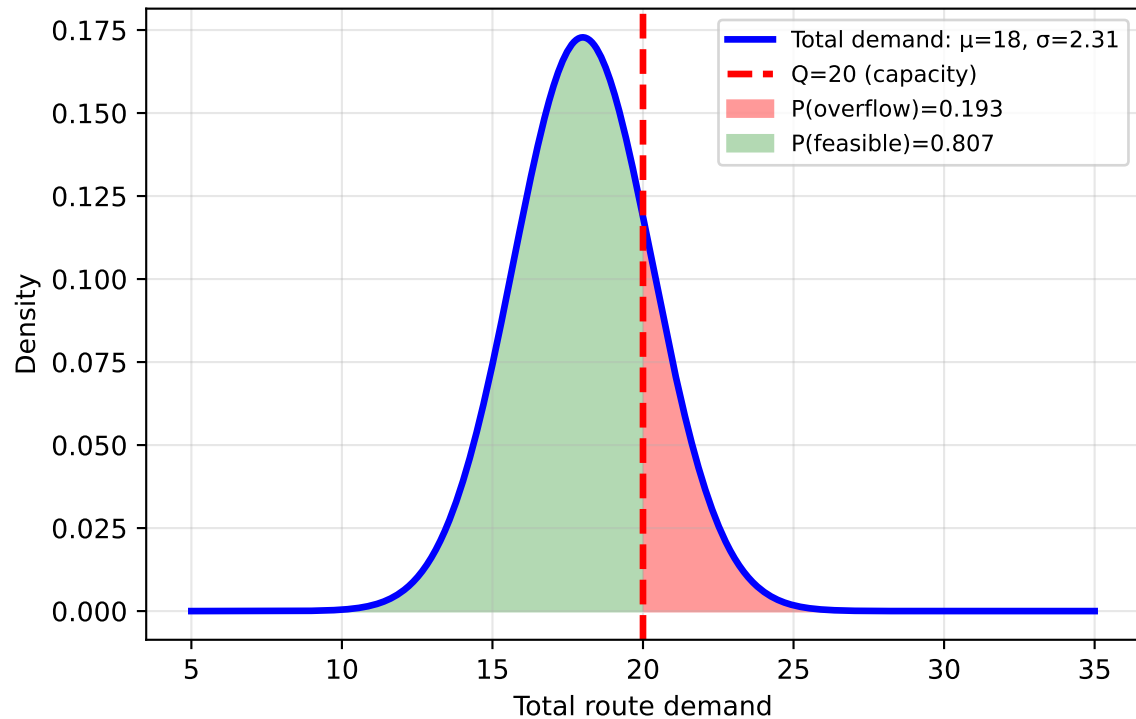
Total Demand Distribution & Chance Constraint
