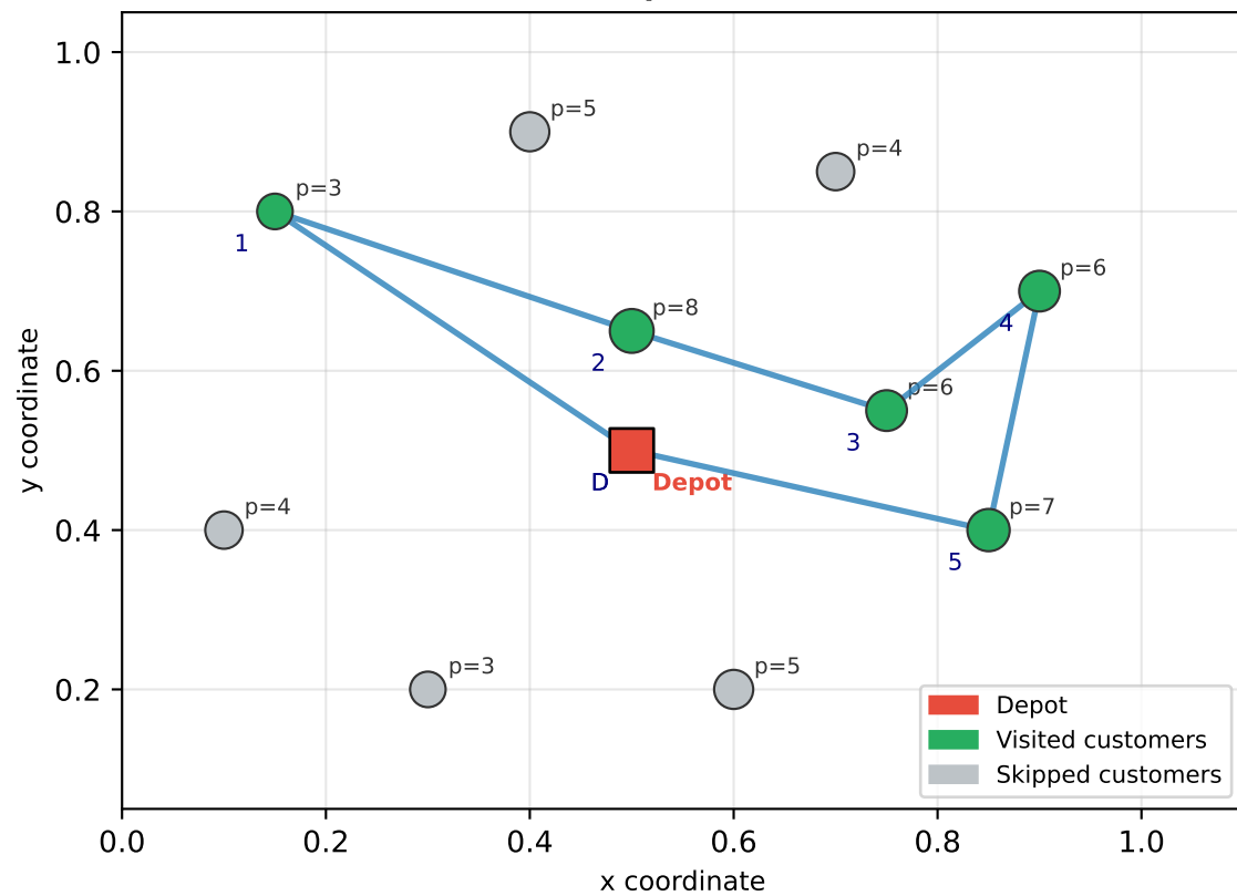
Selected Route (profit collected = 30)
