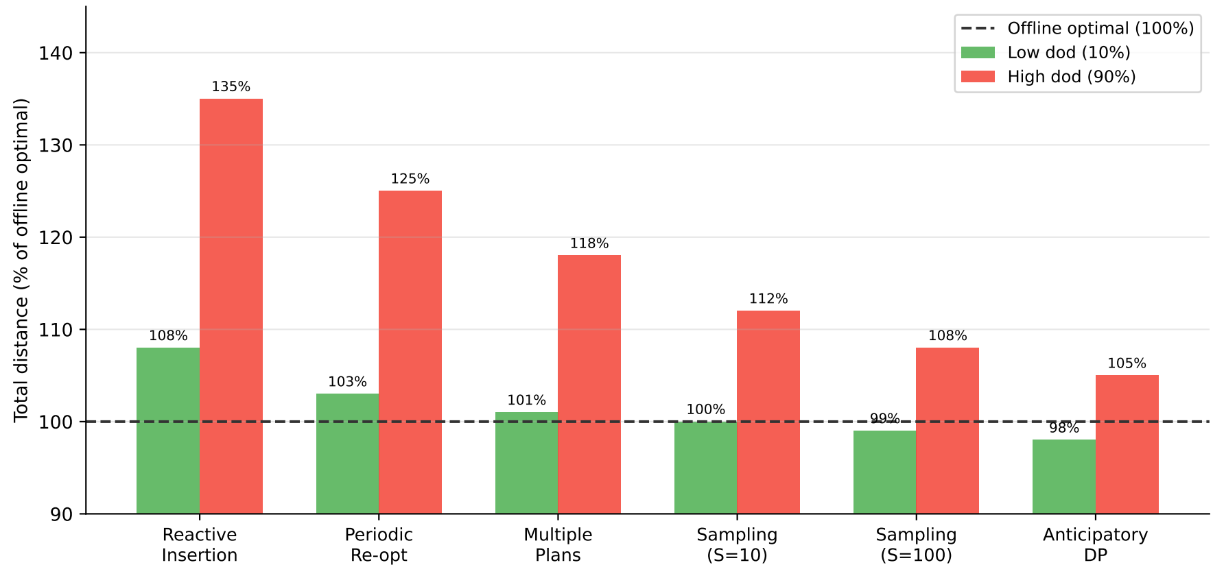
Illustrative Performance Comparison across Dynamic VRP Methods
