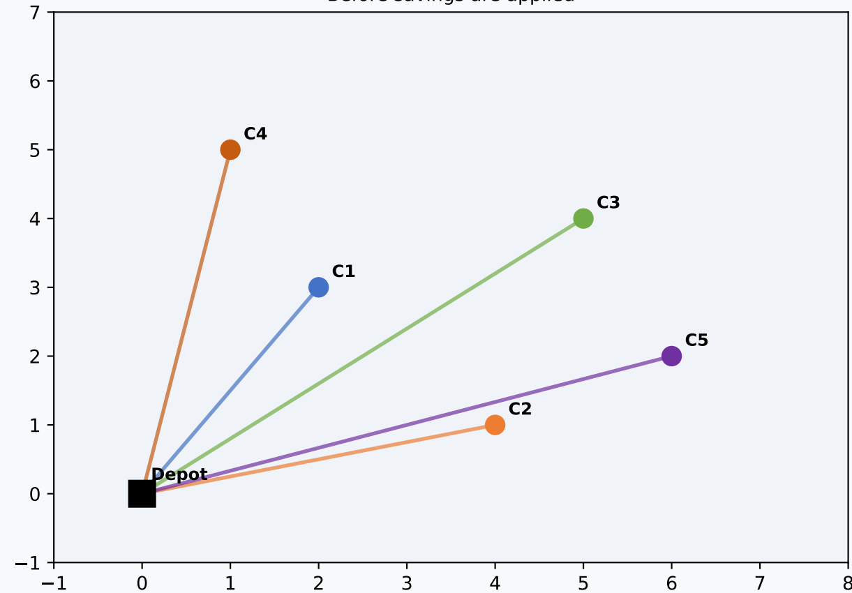
Step 1: Individual (star) routes Before savings are applied
