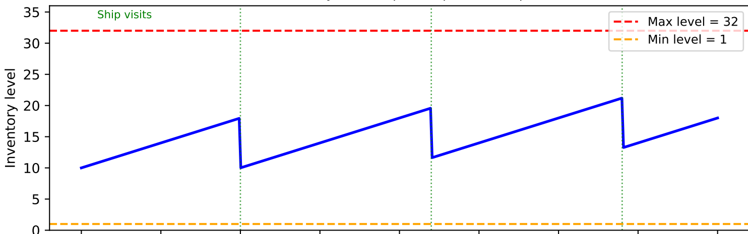
(a) Inventory level at port 4 (production port)
