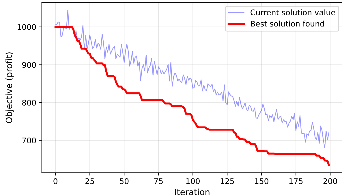
Tabu Search Convergence - Tramp Ship Routing
