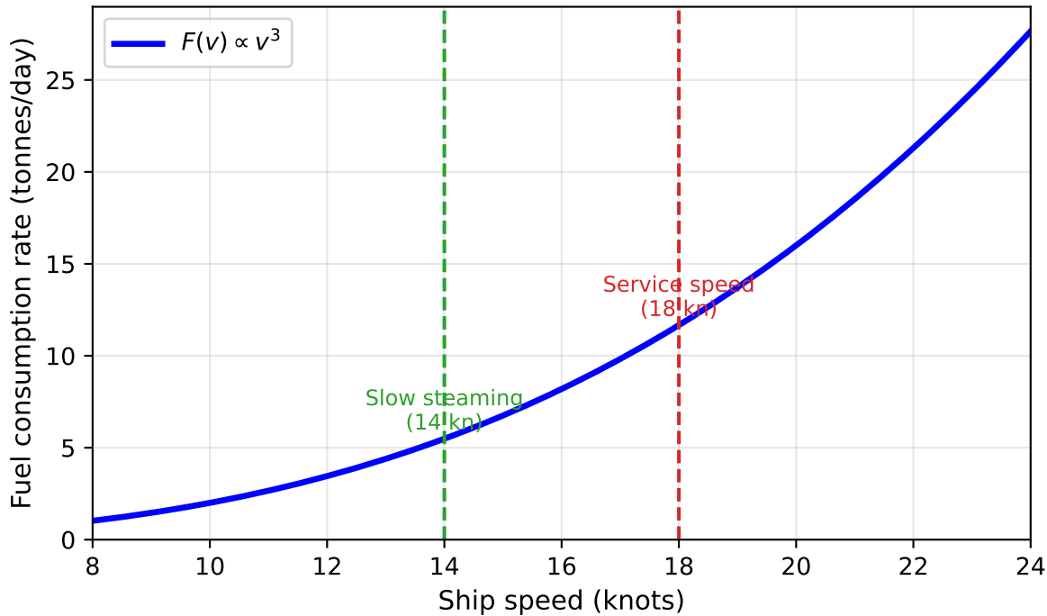
Fuel Consumption vs. Speed (cubic relationship)
