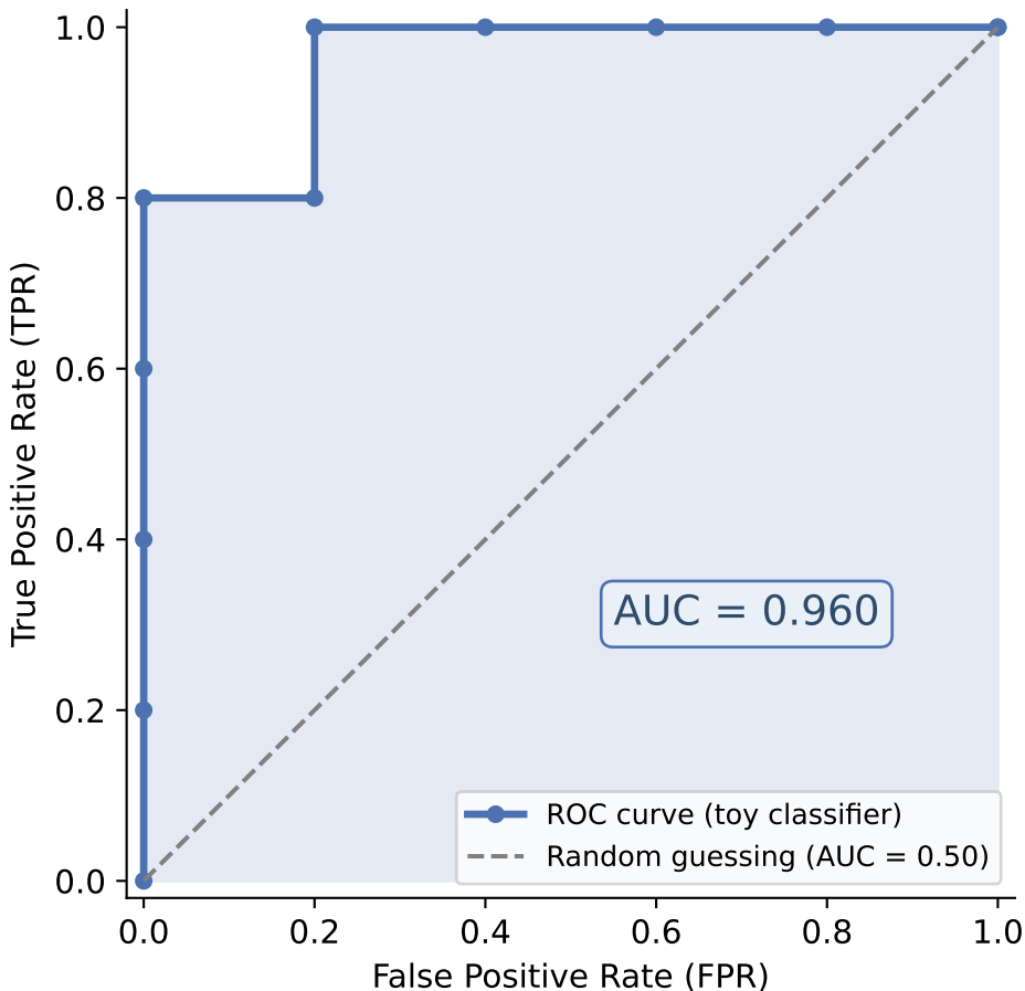
ROC curve and Area Under the Curve (AUC) for a toy binary classifier
