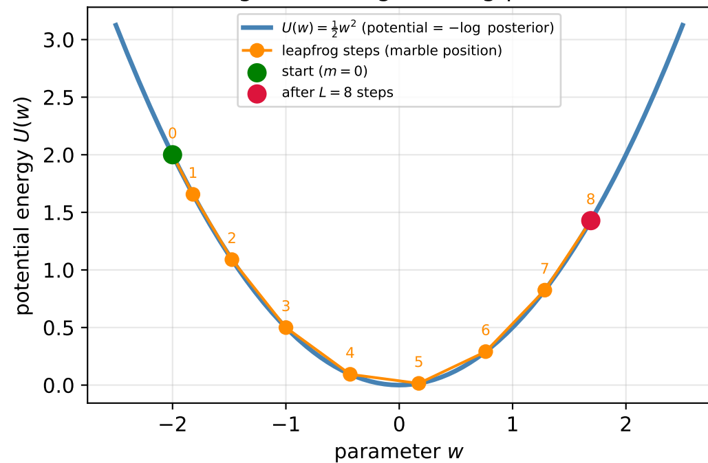
Marble rolling on the negative log-posterior surface
