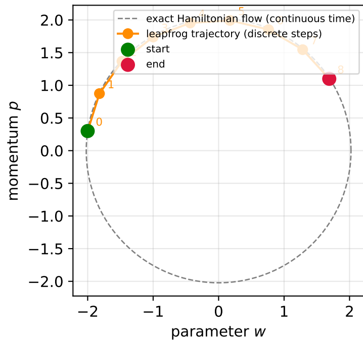
Phase space (w, p) : leapfrog nearly conserves the Hamiltonian
