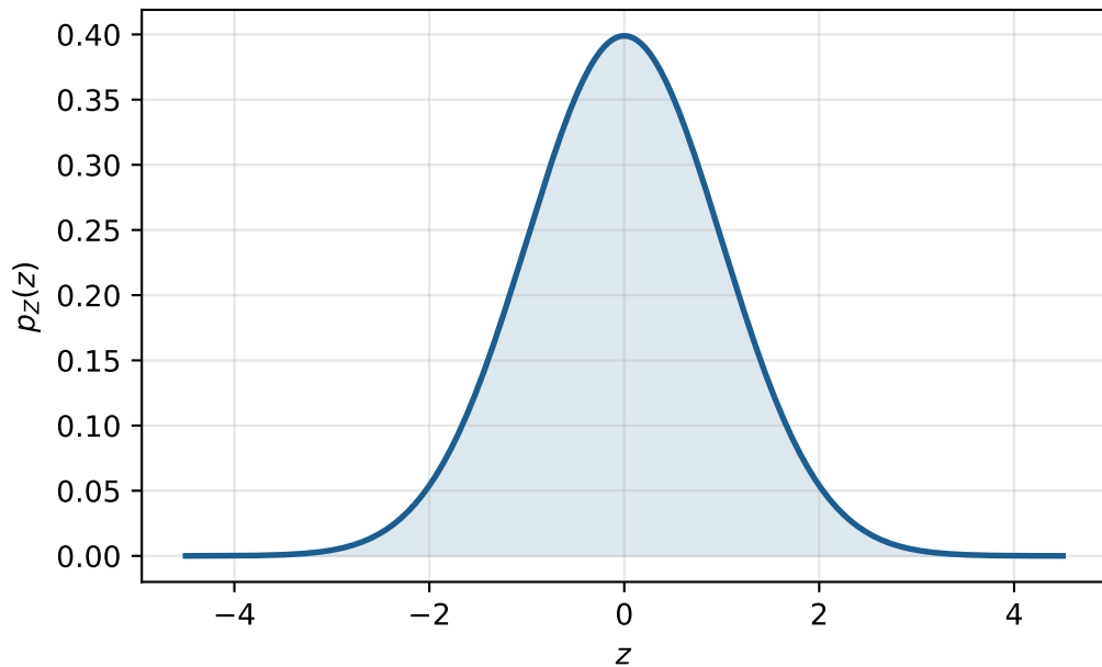
(a) Base density: standard Gaussian
