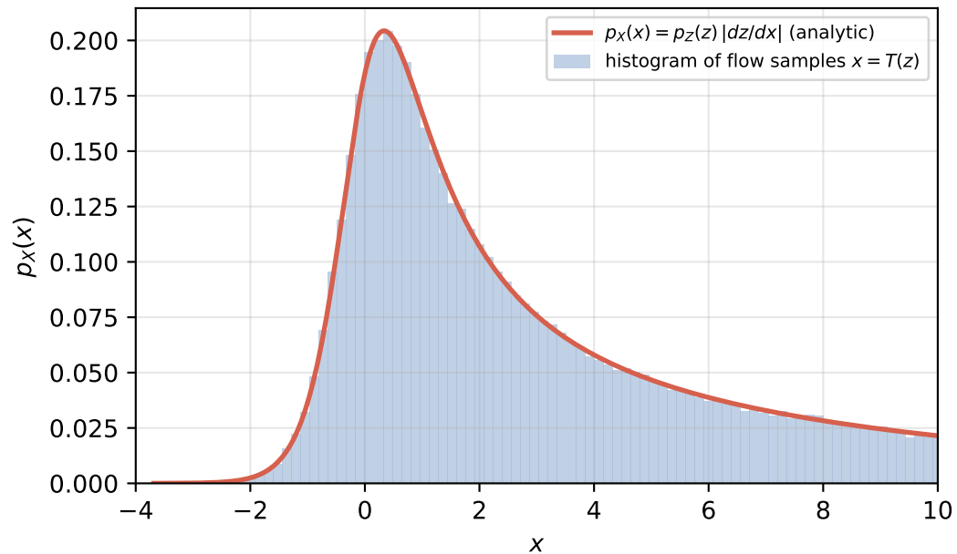
(b) Transformed density: skewed / fat-tailed
