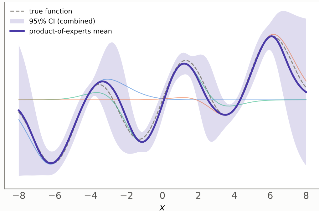
Step 2: combine experts via product-of-experts rule
