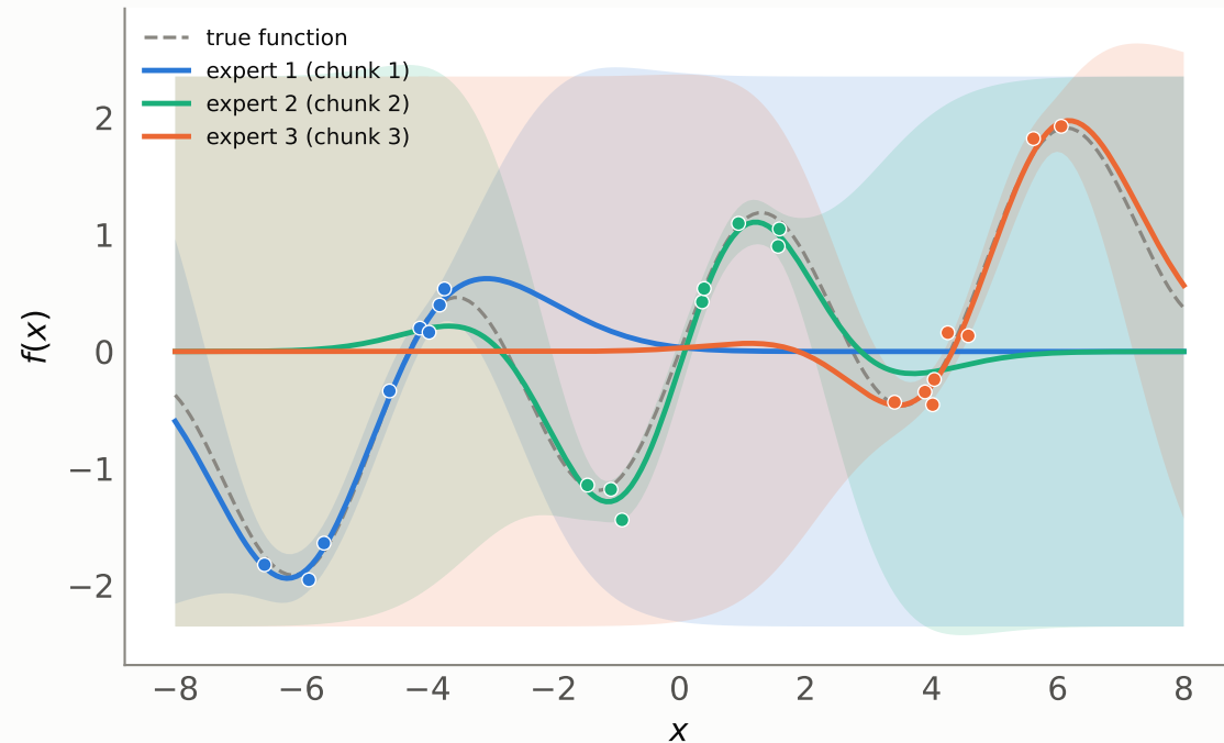
Step 1: fit one small GP "expert" per data chunk
