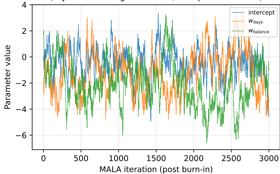
Trace plot: from-scratch MALA (toy 2-feature logistic model, accept rate \approx 0.99 )
