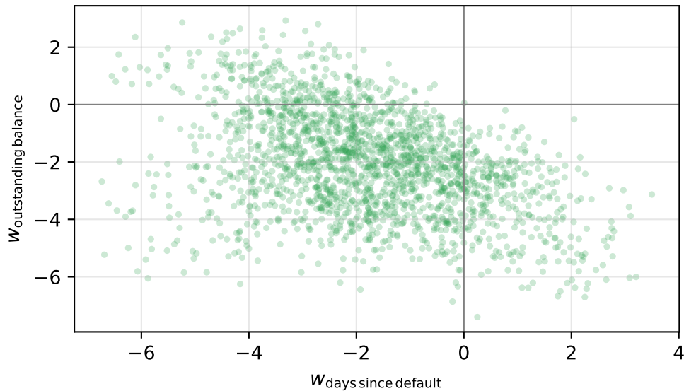
Toy posterior samples (from-scratch MALA, 6 fictional accounts)
