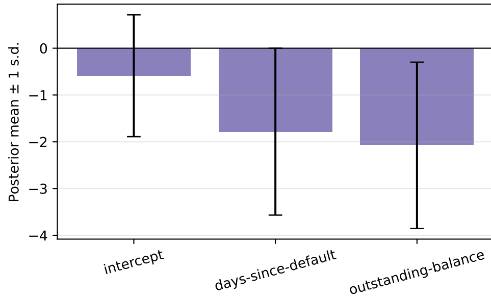
Toy posterior summaries (illustrative ARD-style importance)
