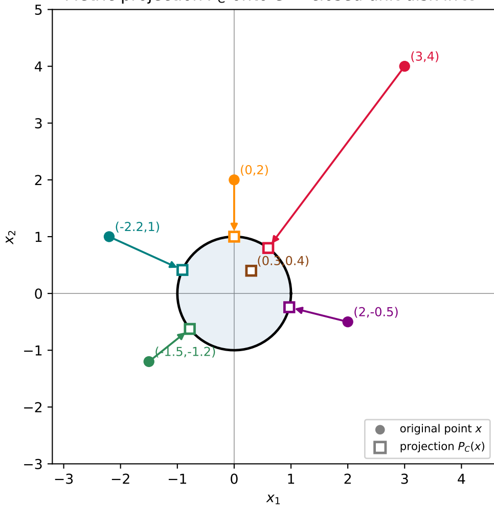
Metric projection P_C onto C = closed unit disk in \mathbb{R}^2
