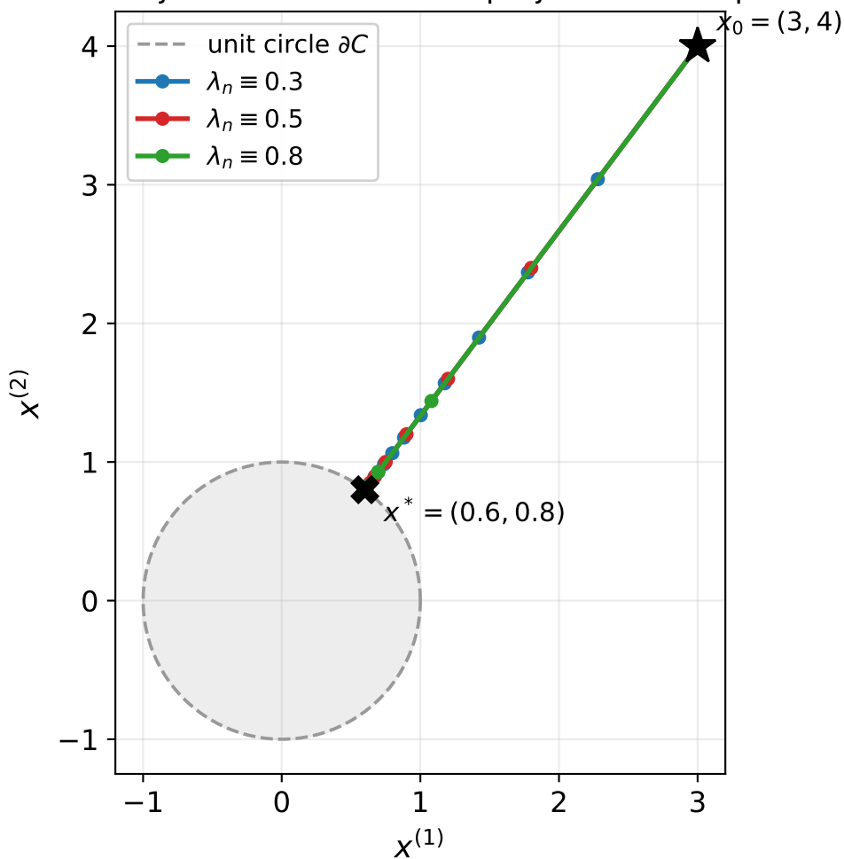
KM trajectories for the disk-projection example
