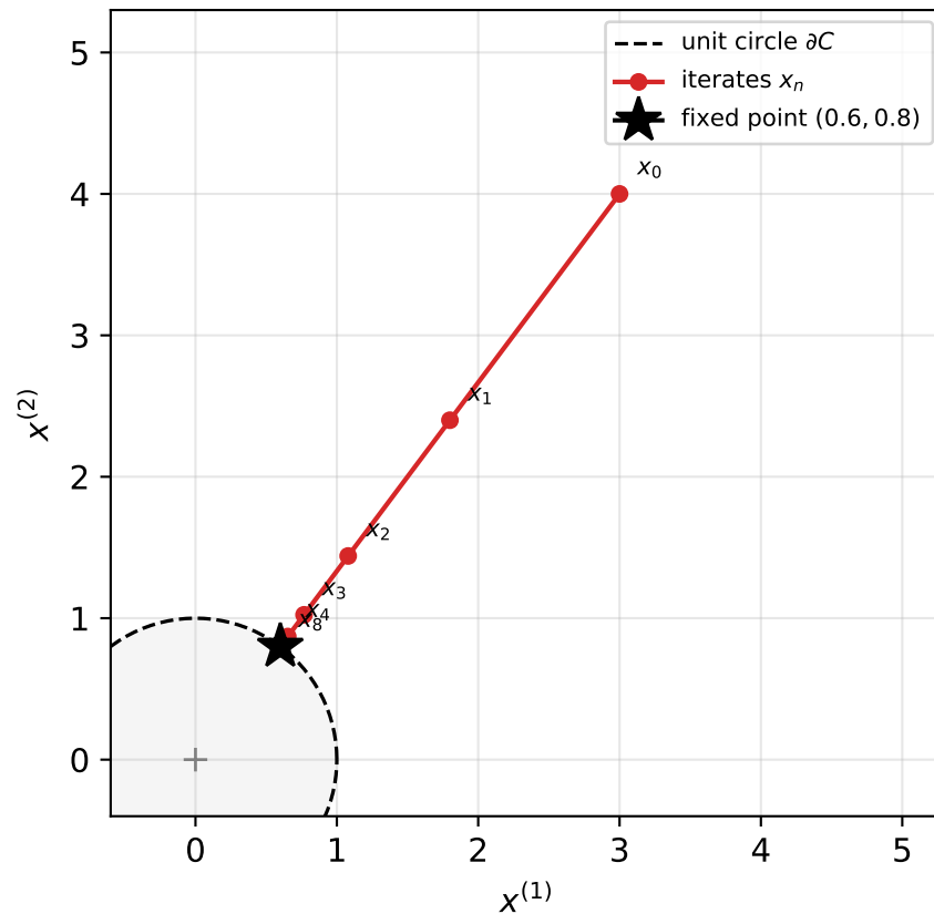
Inertial KM ( \theta_n = 0.2, \lambda_n \equiv 0.5 )
