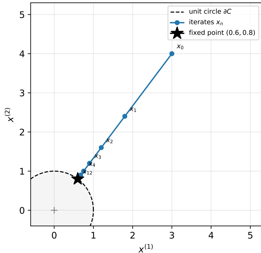
Plain KM ( \lambda_n \equiv 0.5 )
