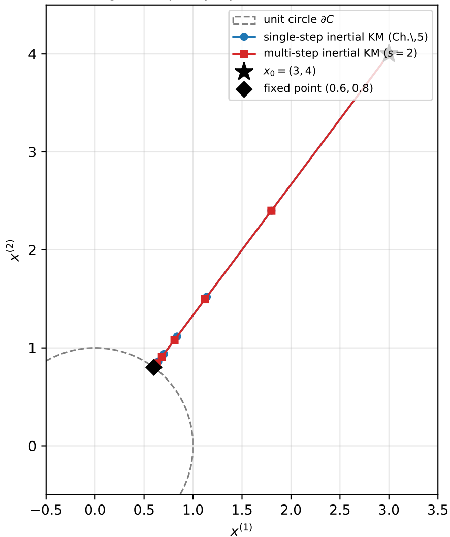
Running example: projection onto the unit disk
