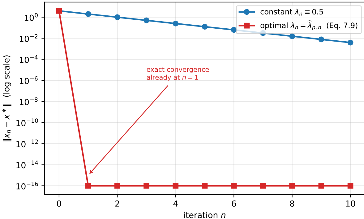
Running example: unit-disk projection, x_0 = (3, 4)
