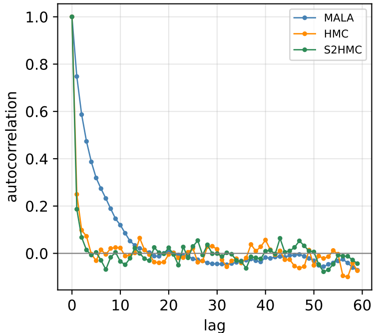
Mixing: autocorrelation decay
