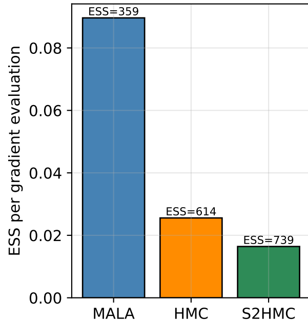
Sampling efficiency
