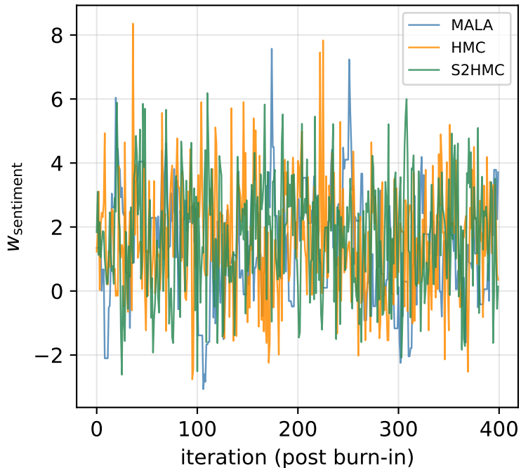
Trace: sentiment coefficient
