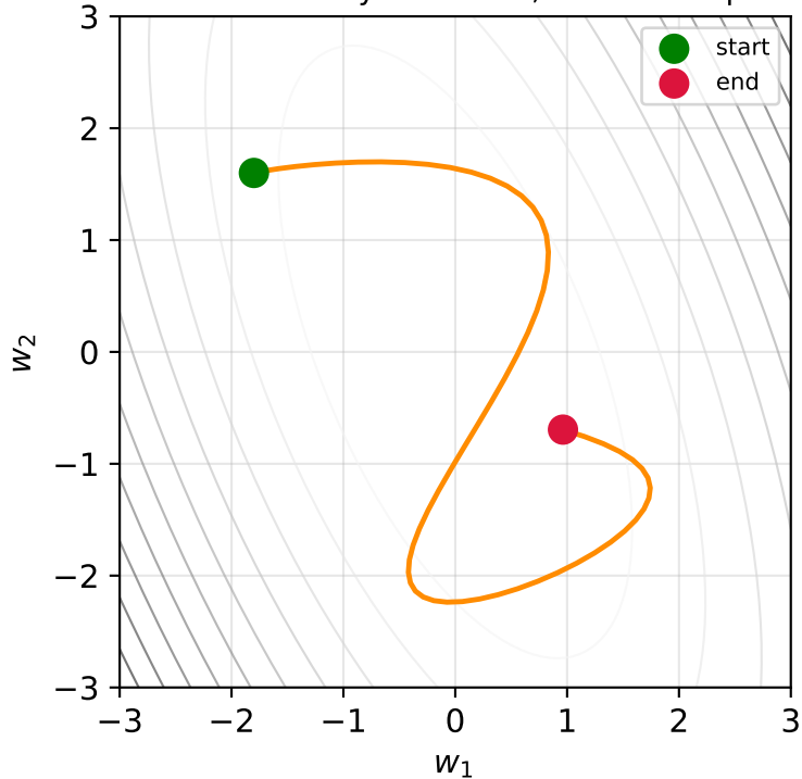
Standard HMC: force field only -- smooth, direct sweeps
