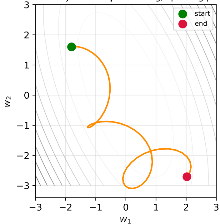
Magnetic HMC: + sideways force \mathbf{Gp} -- curving, spiraling path
