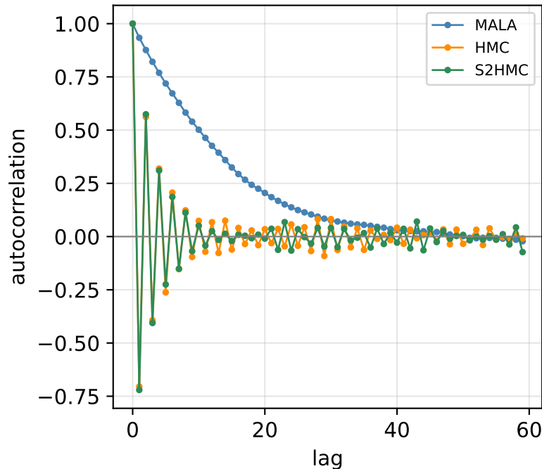
Mixing: autocorrelation decay
