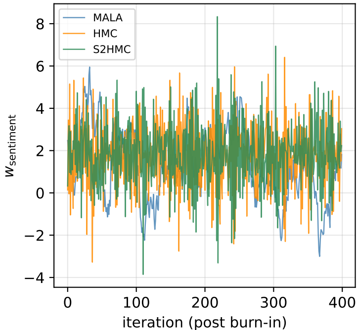
Trace: sentiment coefficient
