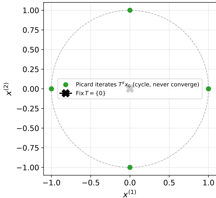
T^k x_0 rotates forever: (x_n) diverges
