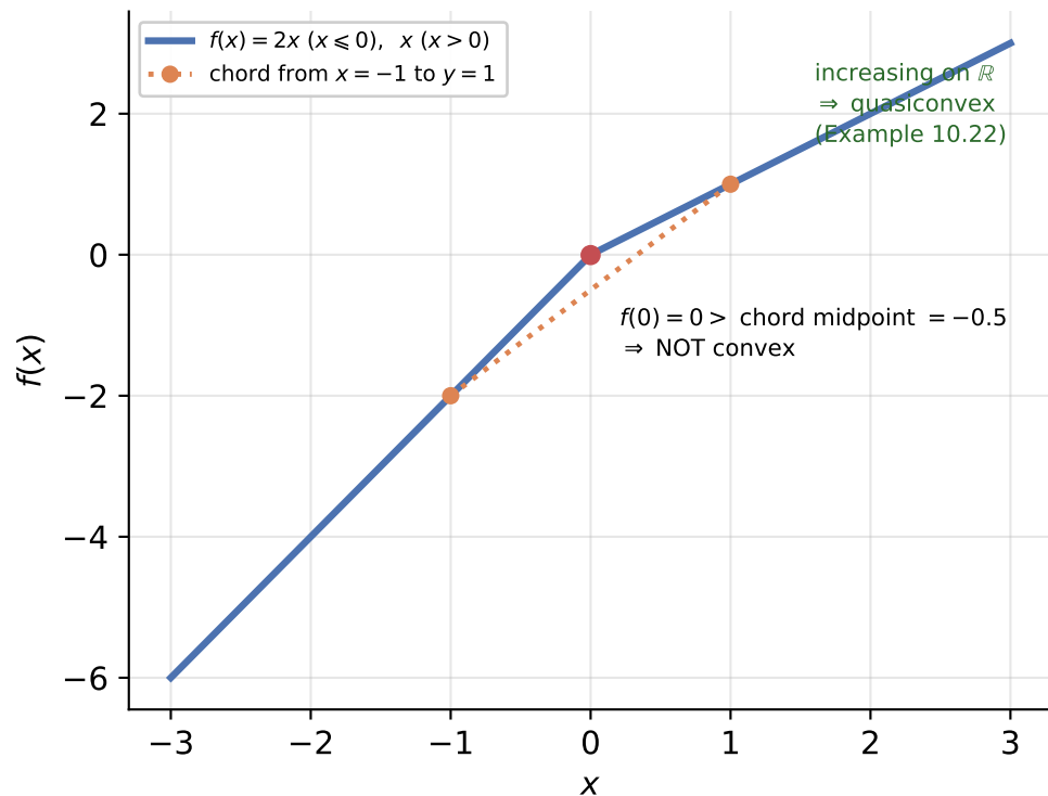
Quasiconvex, not convex (Exercise 10.12)
