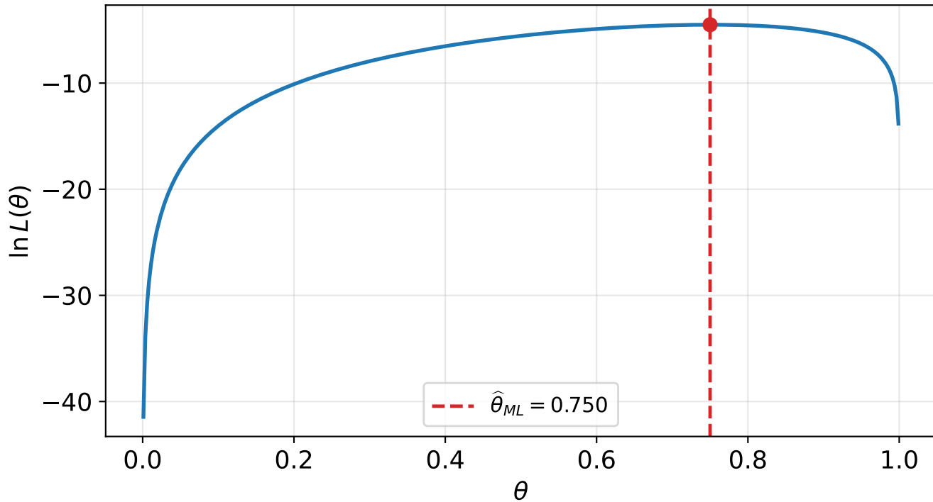
Log-likelihood for n = 8 flips, 6 heads ( x_i = 1 )
