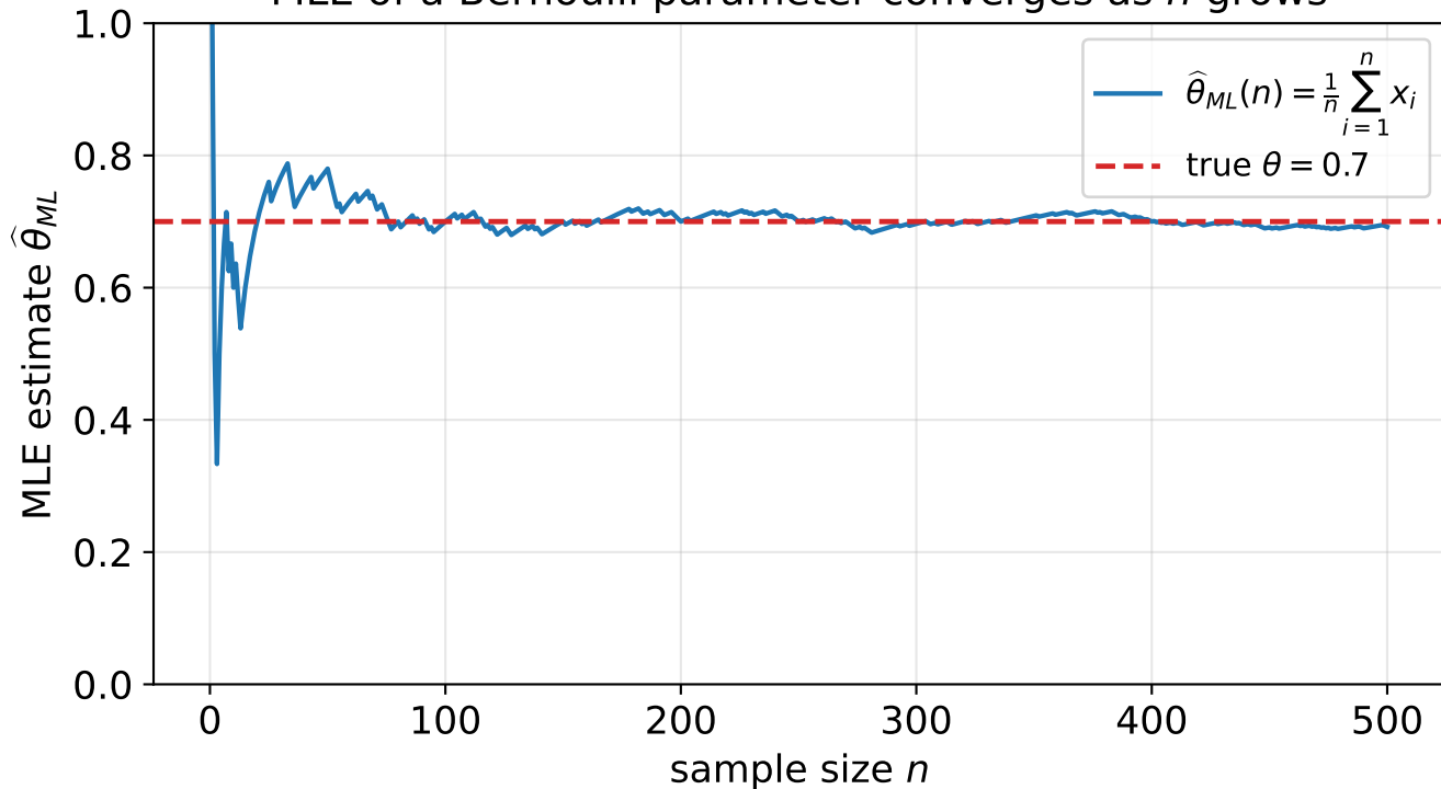
MLE of a Bernoulli parameter converges as n grows
