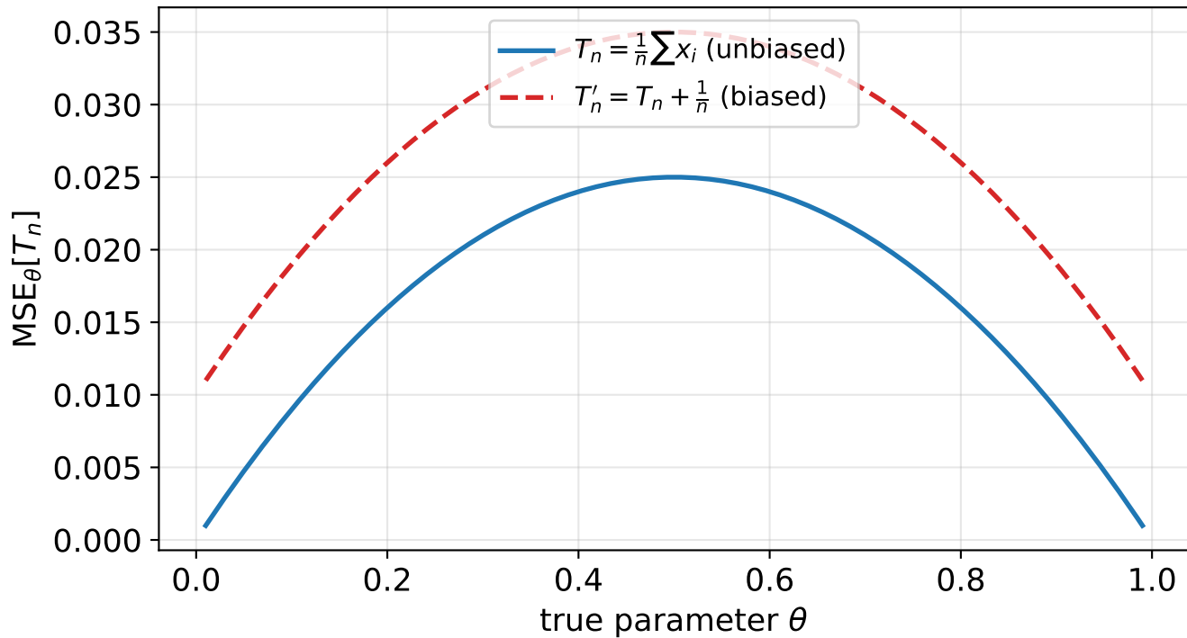
MSE of two estimators of \theta ( n = 10 samples)
