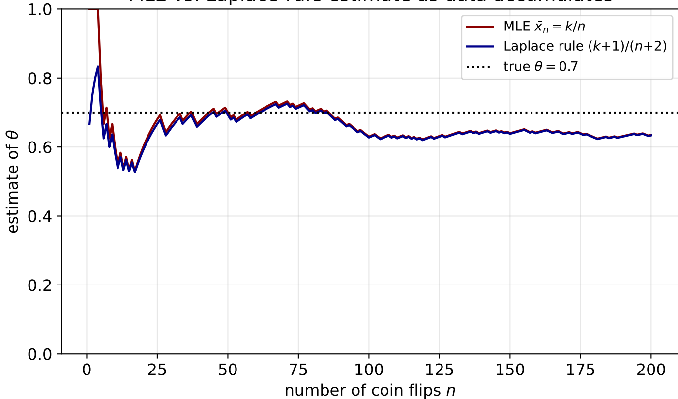
MLE vs. Laplace-rule estimate as data accumulates
