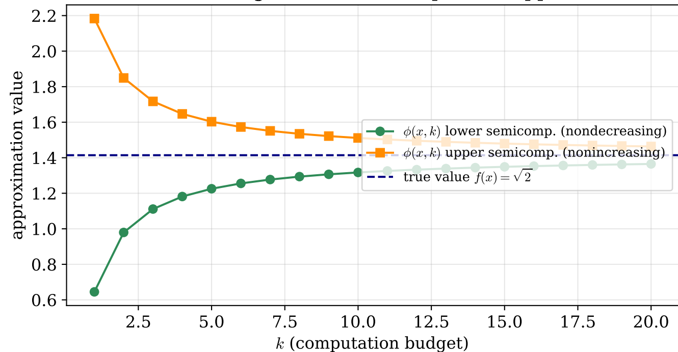
Monotone convergence of semicomputable approximations
