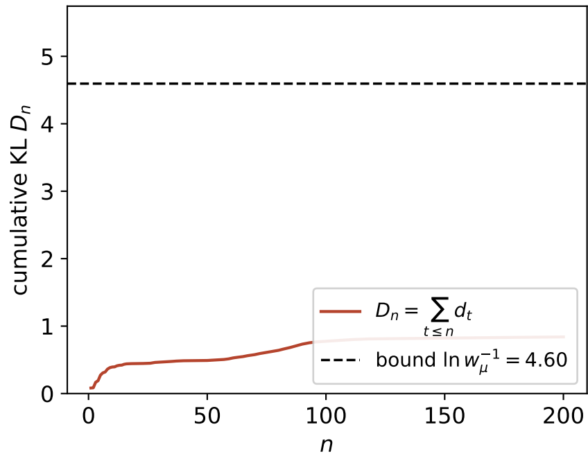
Generalized Solomonoff bound (Thm 3.2.5)
