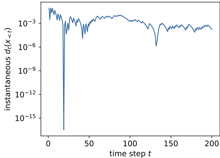
KL distance d_t \rightarrow 0
