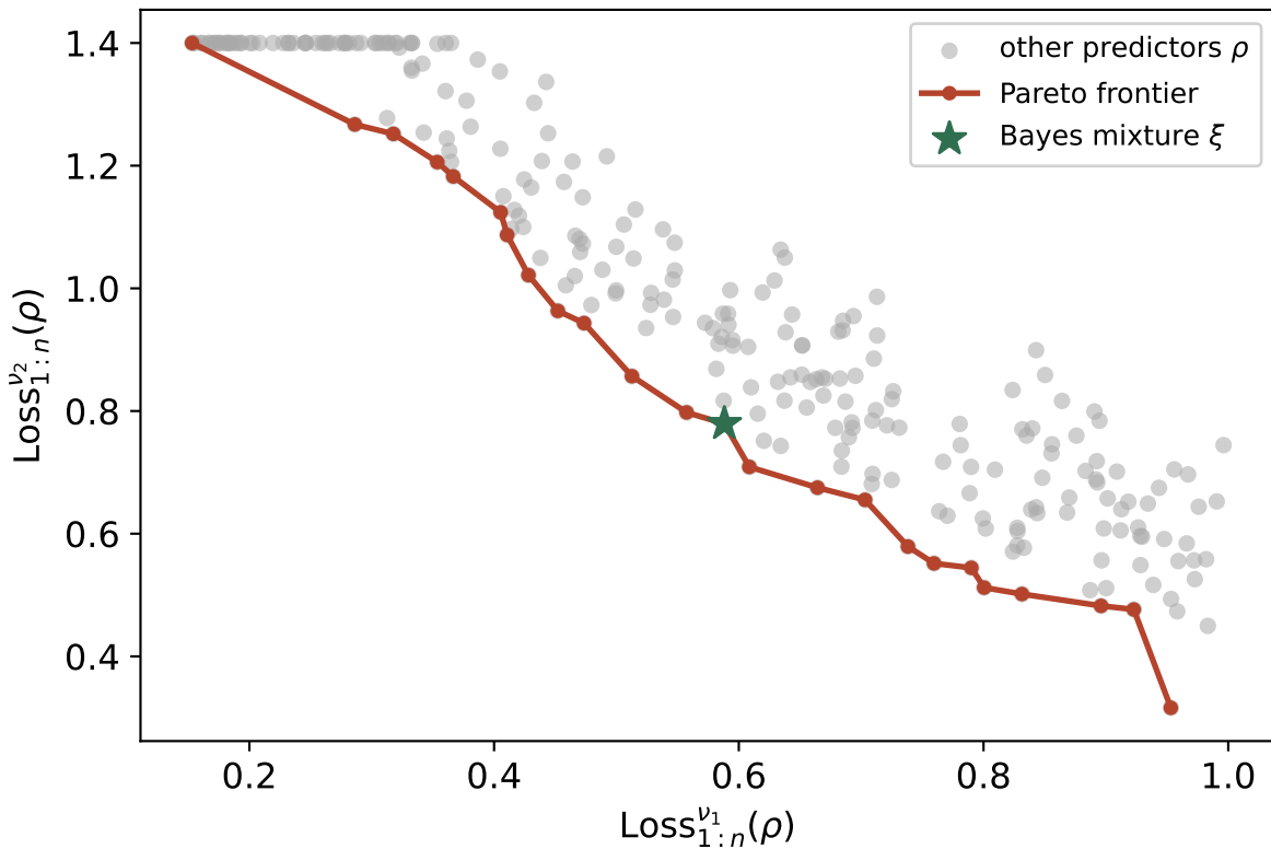
Pareto optimality of \xi (Def. 3.6.1)
