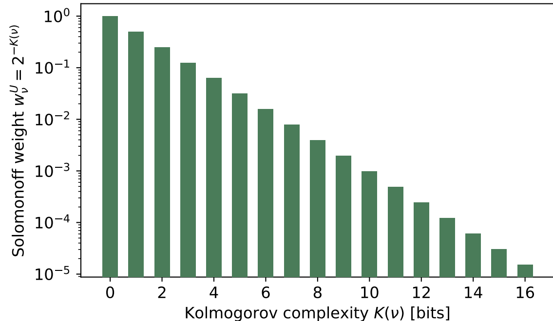
Simplicity bias of the Solomonoff prior
