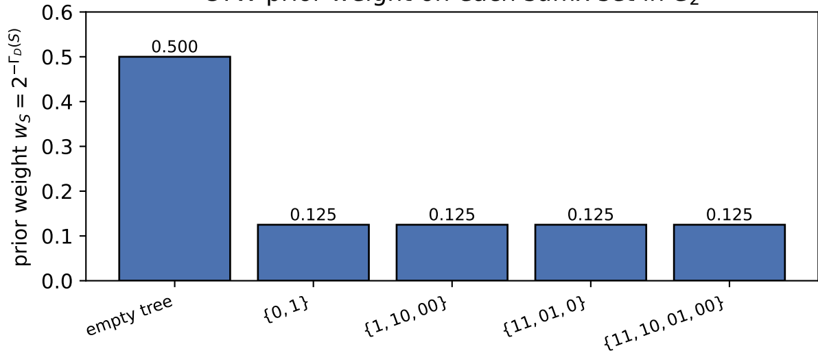
CTW prior weight on each suffix set in C_2
