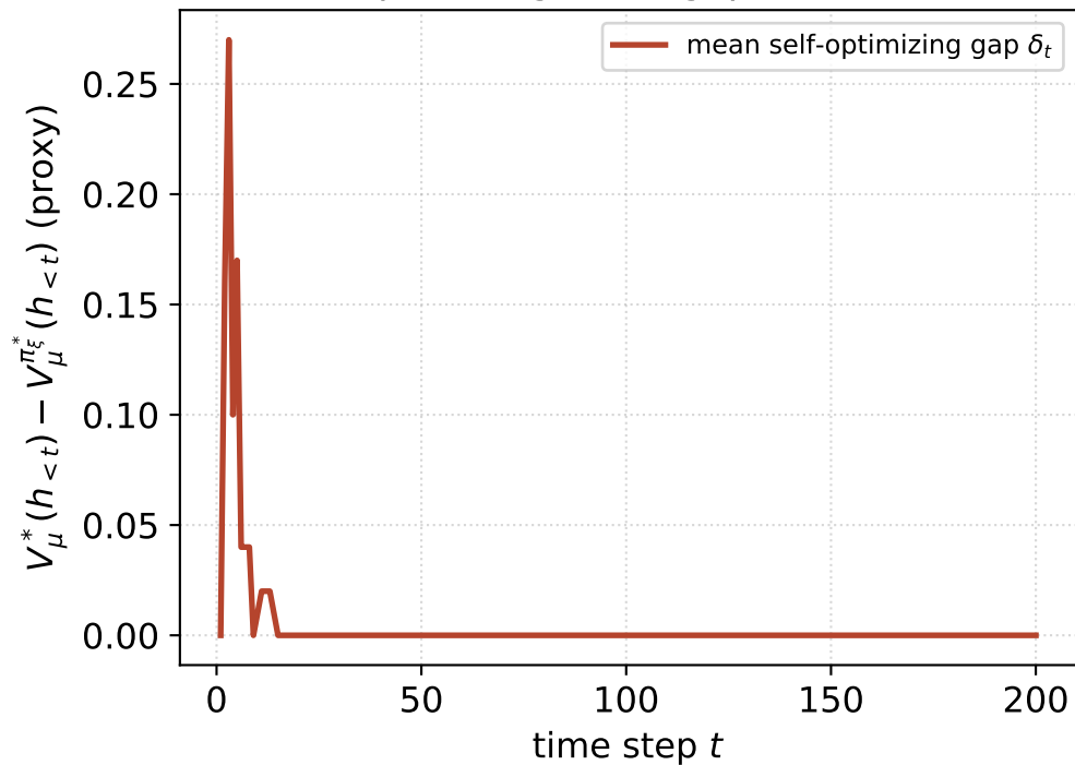
Self-optimizing value gap (Thm 7.3.6)
