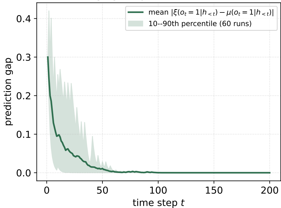
Merging of opinions (Thm 7.2.6)
