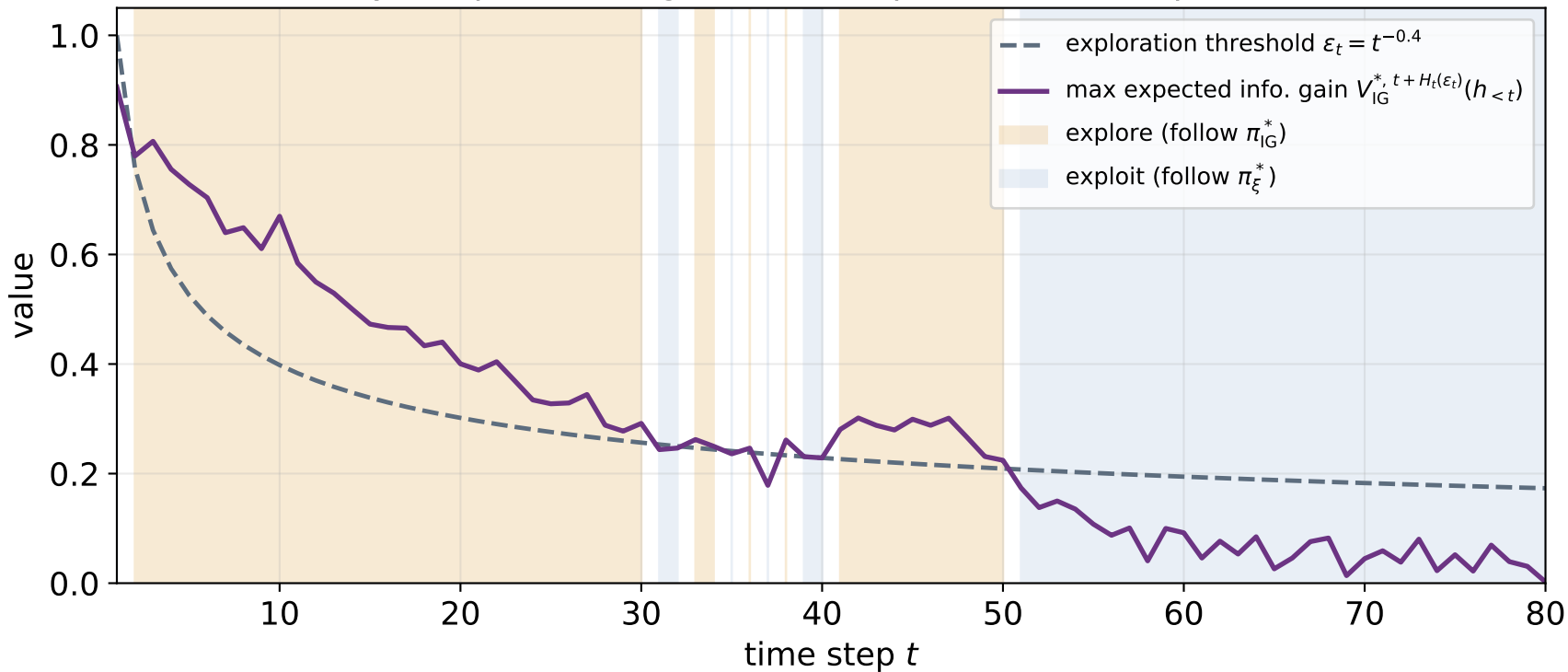
BayesExp: switching between exploration and exploitation
