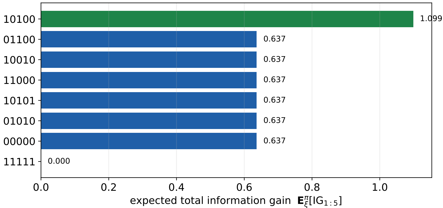
KSA agent's ranking of length-5 action prefixes \dot{a}_{1:5} ( \dot{a}_{1:5} = 10100 wins -- matches Example 9.3.11)
