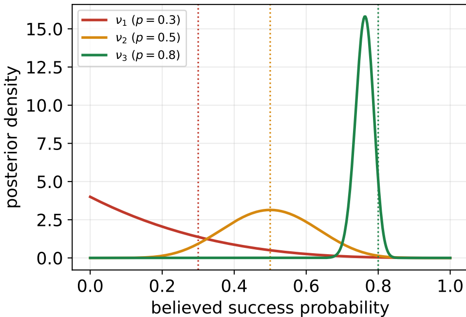
Posterior over each v_i after t = 300 steps
