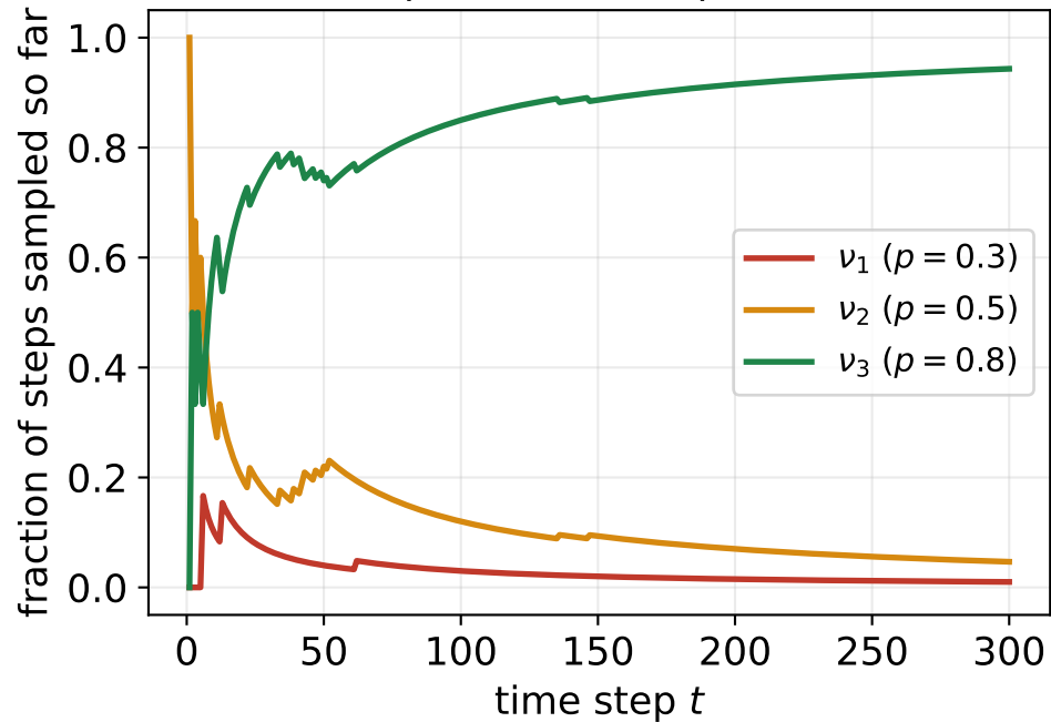
Thompson sampling: which environment gets sampled from the posterior
