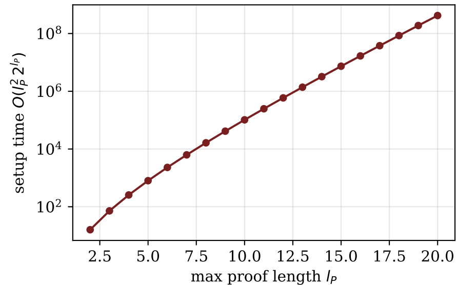
Setup phase cost (checking all candidate proofs)
