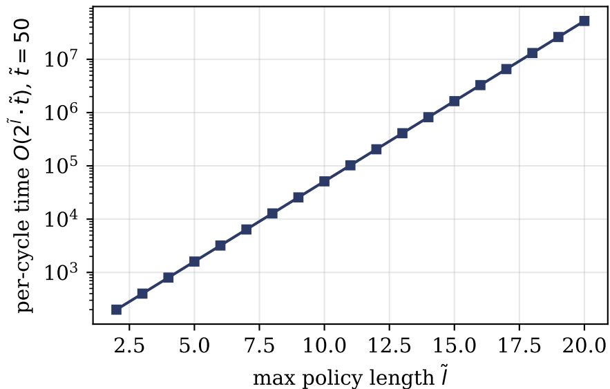
Interaction-loop cost per cycle (running every \tilde{\pi} \in \Pi_{VA} )
