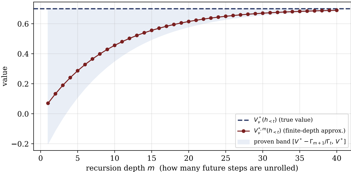
Estimability of V_v^* : the finite-depth approximation gap is bounded by \Gamma_{m+1}/\Gamma_t \rightarrow 0 (numeric illustration, \gamma_k = 0.9^k , t=1 )
