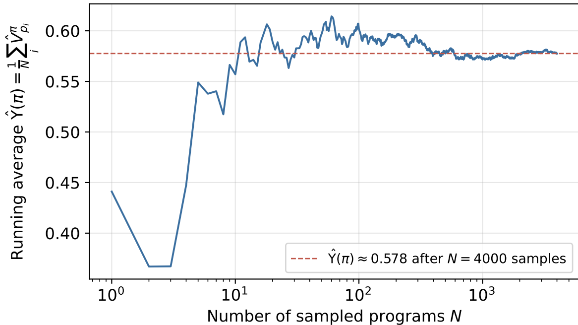
AIQ estimator: empirical average converges as N grows
