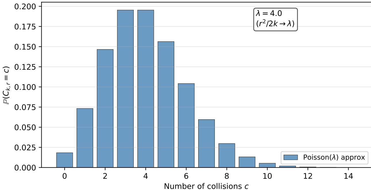
Collision Count: Poisson Approximation ( \lambda = r^2/2k )
