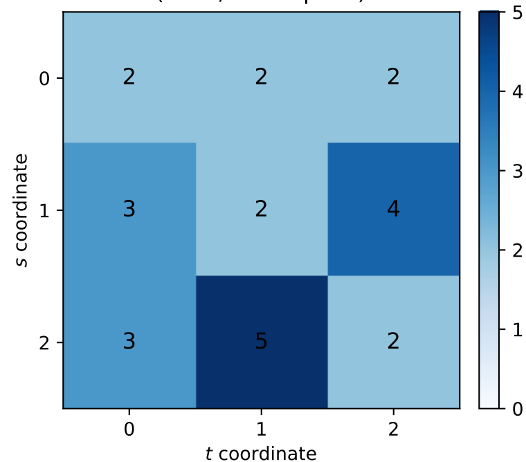
Frequency of Pairs Test: Set A (random) ( L = 3 , r = 25 pairs)
