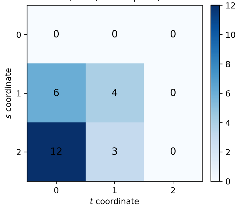
Frequency of Pairs Test: Set C (quasi-random) ( L = 3 , r = 25 pairs)
