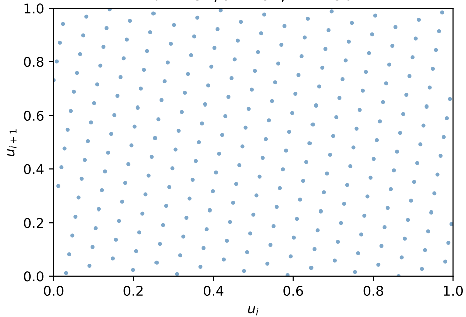
LCG pairs (u_i, u_{i+1}) a = 137, c = 187, M = 256
