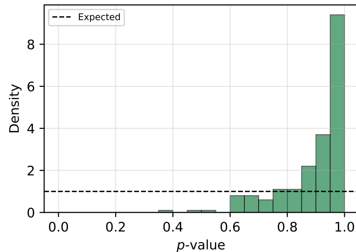
Quasi-random (large p -values)
