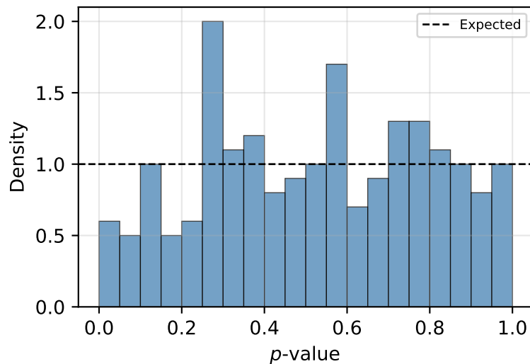
Good PRNG (uniform p -values)
