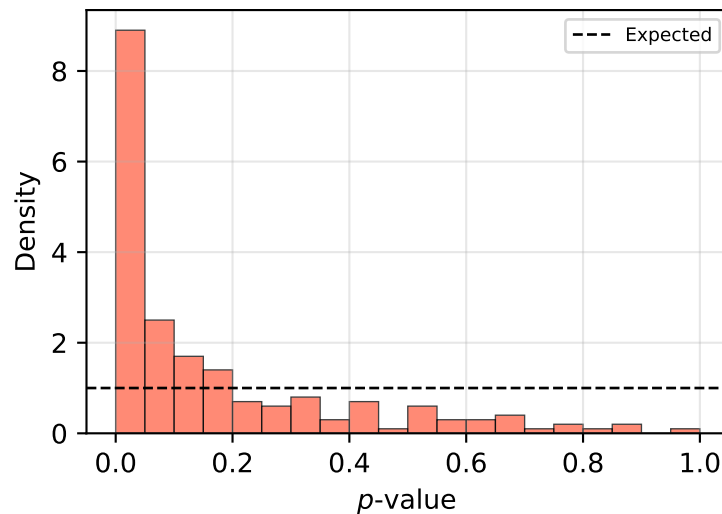
Bad PRNG (small p -values)
