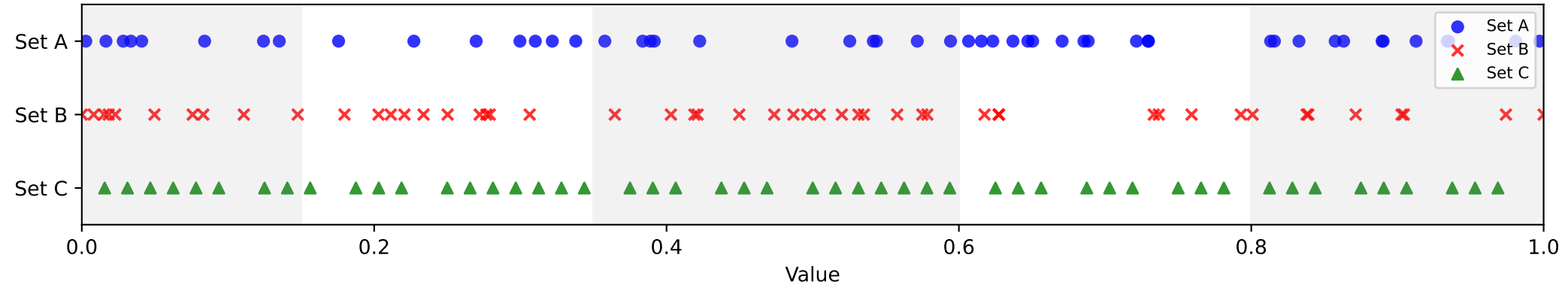
Three sets of n = 50 points from [0, 1) : A (blue), B (red), C (green)
