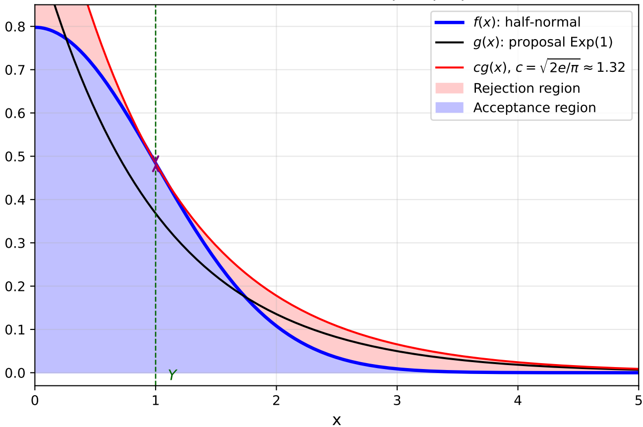
AR-c: Half-Normal from Exp(1) proposal
