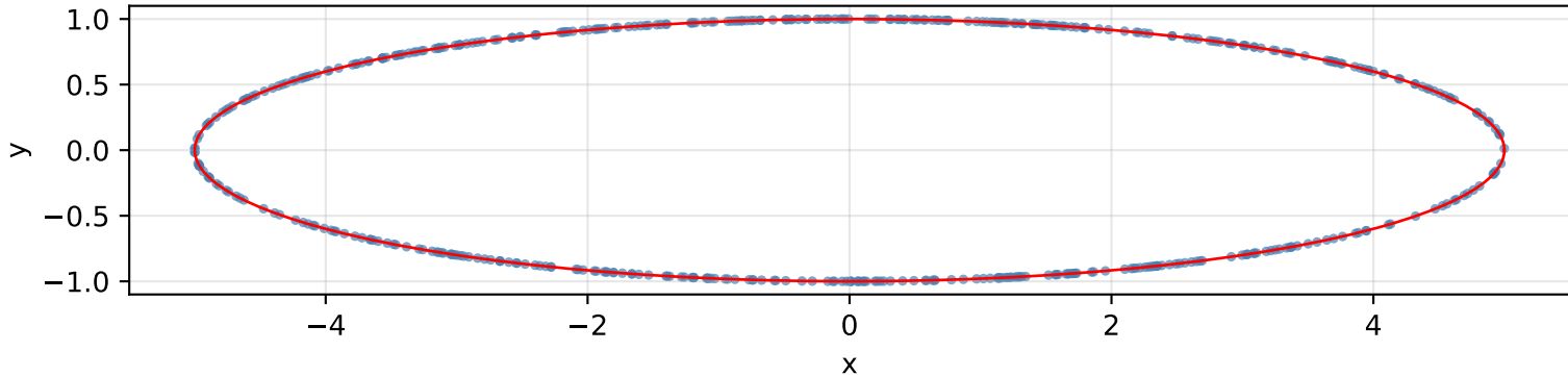
Uniform random points on ellipse (x/5)^2 + y^2 = 1
