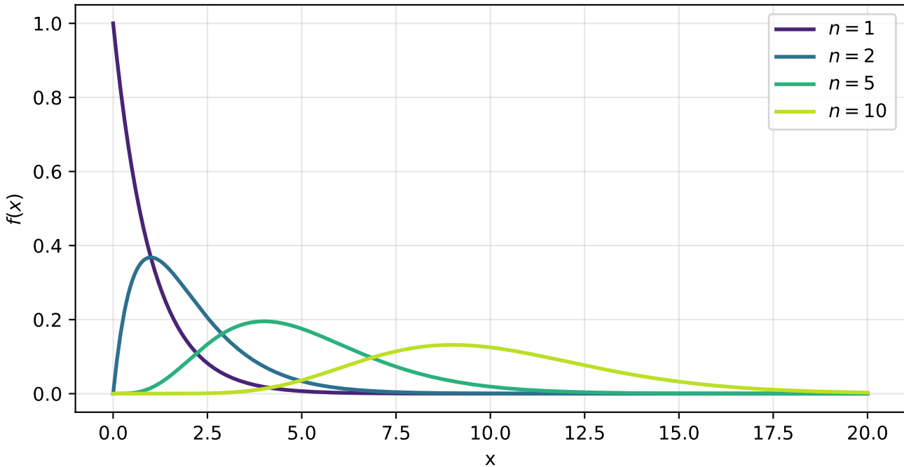
Erlang( n, \lambda = 1 ) = sum of n i.i.d. \text{Exp}(\lambda)
