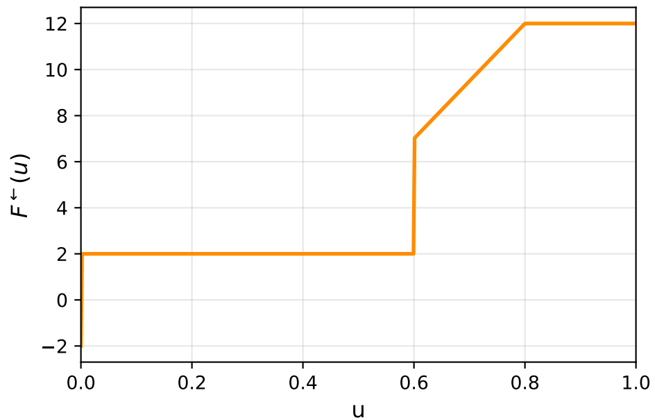
Generalised Inverse F^{\leftarrow}
