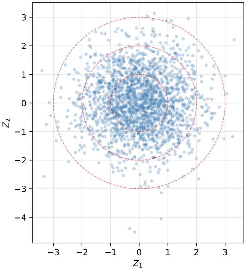
Marsaglia-Bray: 2000 standard normal pairs
