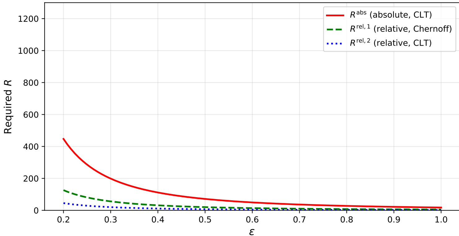
Required replications to estimate \pi ( \delta = 0.01 )
